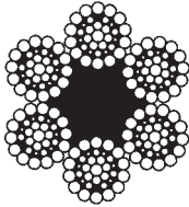
6x36 Warrington Seale with Fiber Core
