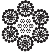
6x36 Warrington Seale with IWRC
